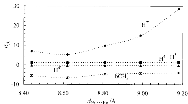
Fig. 11 Calculated R_{ik} factors for pairs H^5-H^k ( k = 3, 4, 4', 7' ) and H^5 -b-CH 2 in the crystal structure of [\text{Ln}_2(\text{L}^5 - 2\text{H})_3] (intermetallic distance d varies from 8.4 to 9.2 Å, see Table 4).
