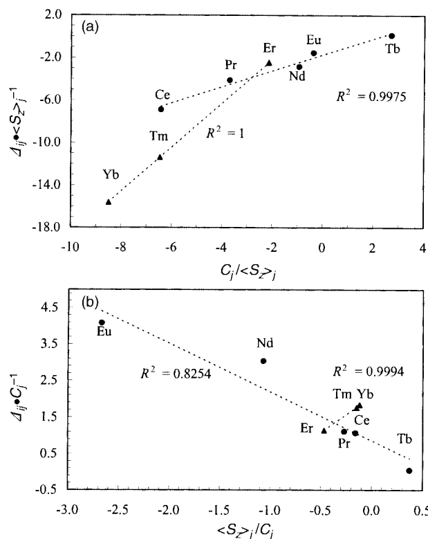
Fig. 9 Plots of (a) A_{ij} \cdot \langle S_z \rangle_j^{-1} vs. C_j \cdot \langle S_z \rangle_j^{-1} and (b) A_{ij} \cdot C_j^{-1} vs. \langle S_z \rangle_j \cdot C_j^{-1} for H 4 in [\text{Ln}_2(\text{L}^5 - 2\text{H})_3] (water, 298 K).
