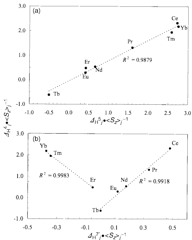
Fig. 10 Plots of \Delta_{ij} \cdot \langle S_{zj} \rangle_j^{-1} vs. \Delta_{kj} \cdot \langle S_{zj} \rangle_j^{-1} according to eqn. (13) for (a) H^4-H^5 and (b) H^4-H^7 in [\text{Ln}_2(\text{L}^5 - 2\text{H})_3] (water, 298 K).
