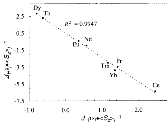
Fig. 7 Plot of A_{ij} \cdot \langle S_z \rangle_j^{-1} vs. A_{kj} \cdot \langle S_z \rangle_j^{-1} according to eqn. (8) for H 9 –H 12 in [\text{LnCo}(\text{L}^4)_3]^{6+} (acetonitrile, 298 K).
